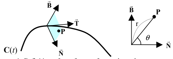
Figure 4. Definition of a reference frame along the space curve C(t) . The parametric coordinate for a point P is given as (r, \theta, t) , where \theta is defined as the angle around the tangent vector \vec{T} , starting from the principal normal \vec{N} .
